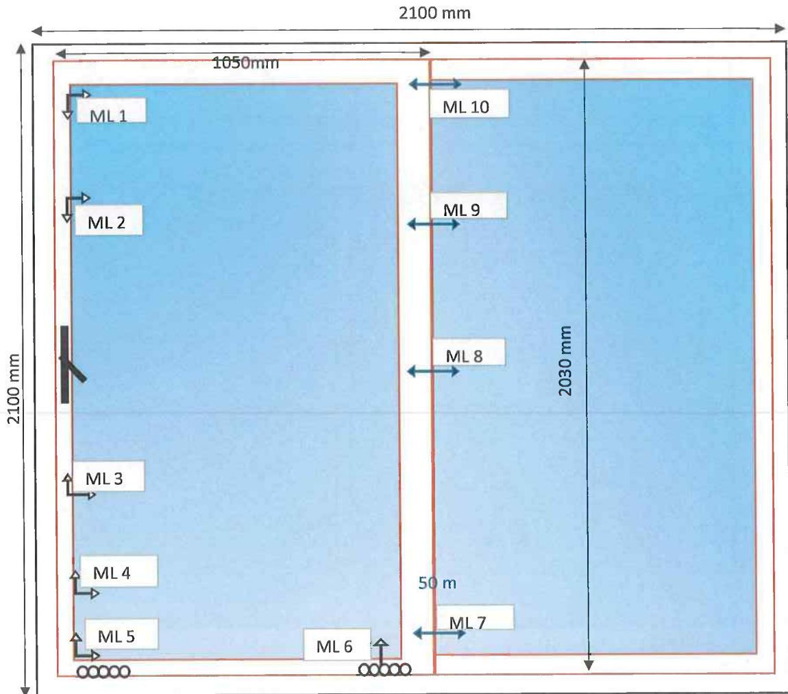
Mechanical Loads
